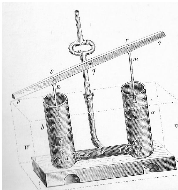
Heronova brizgalna
